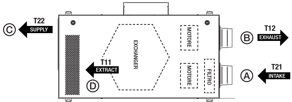
Fig. 7.a Temperature probes
