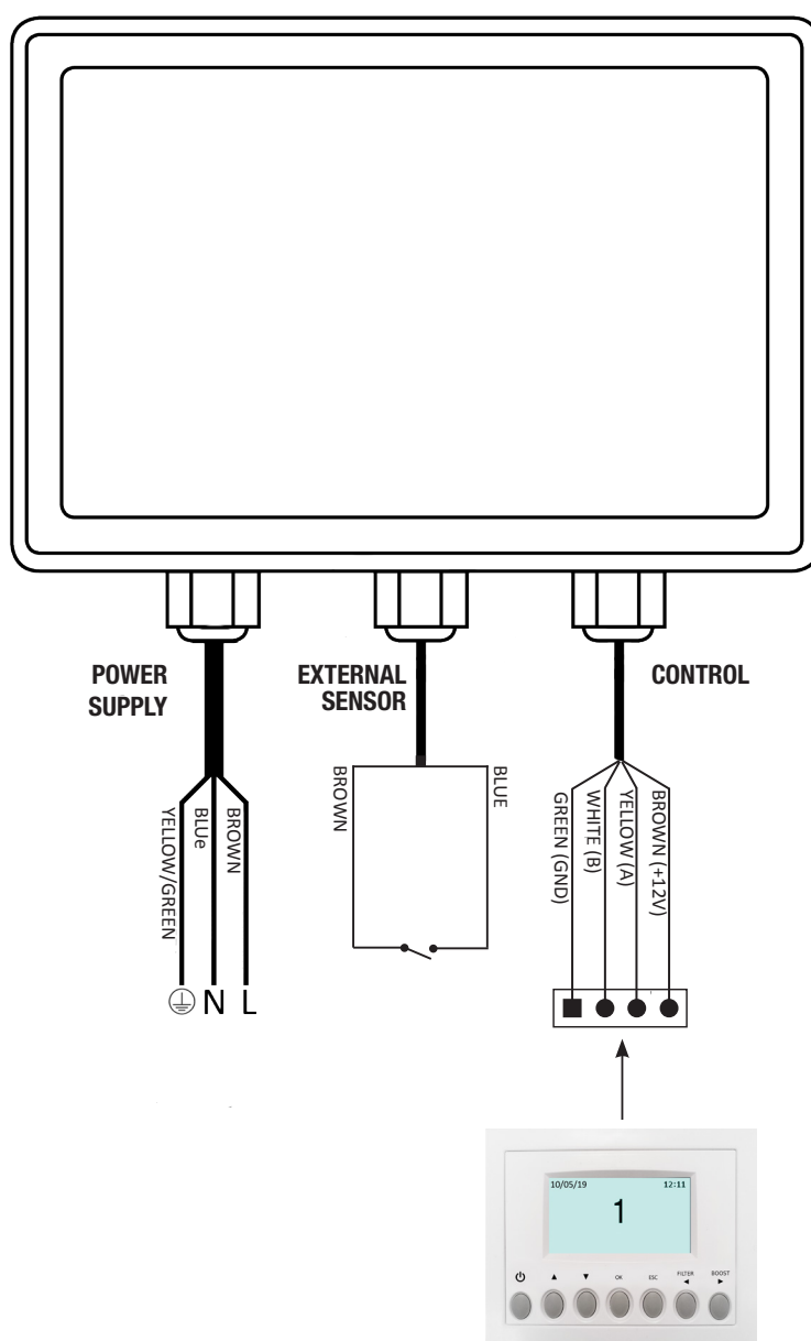
Fig. 5.g Electrical connection
