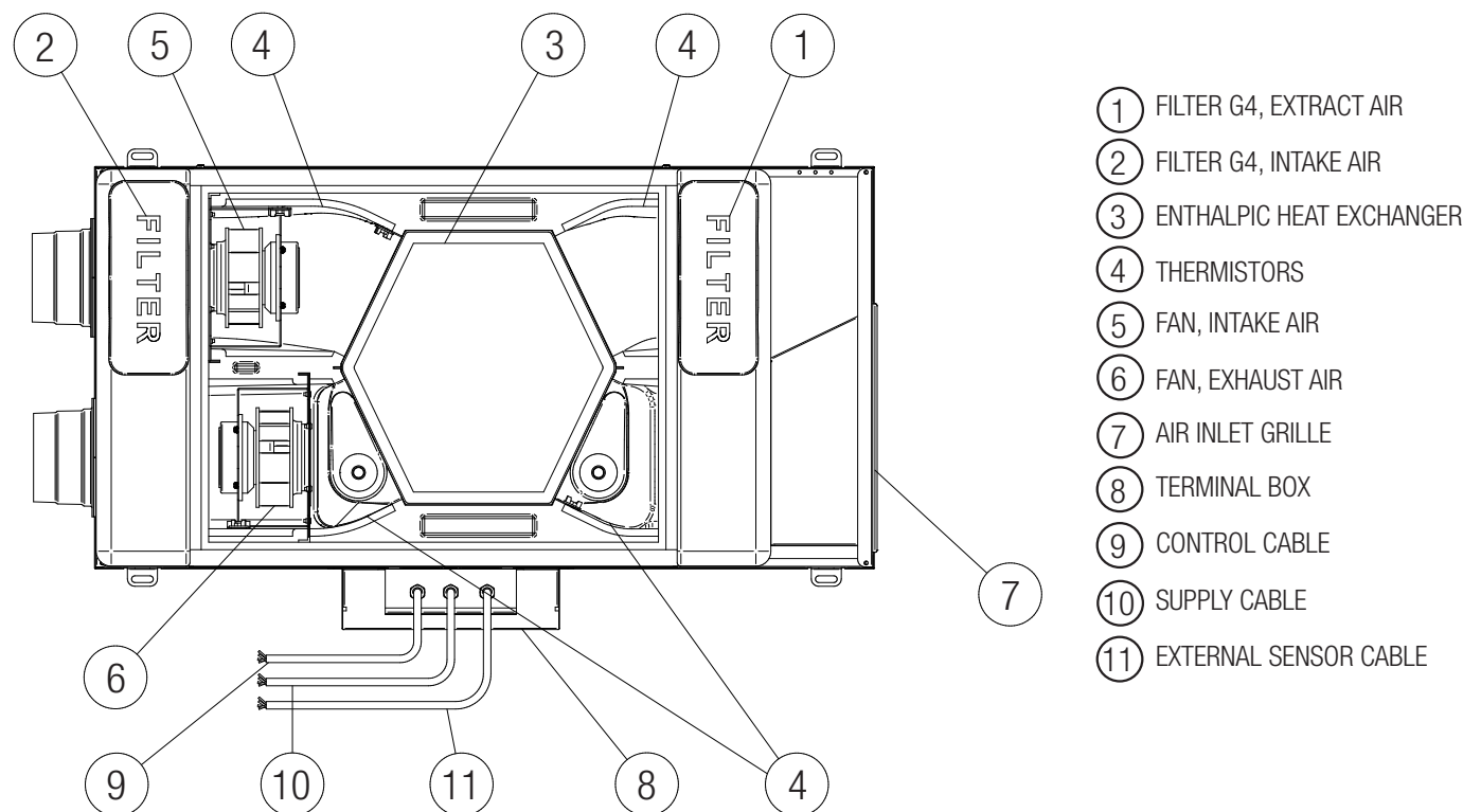
Fig. 8.a Internal components
