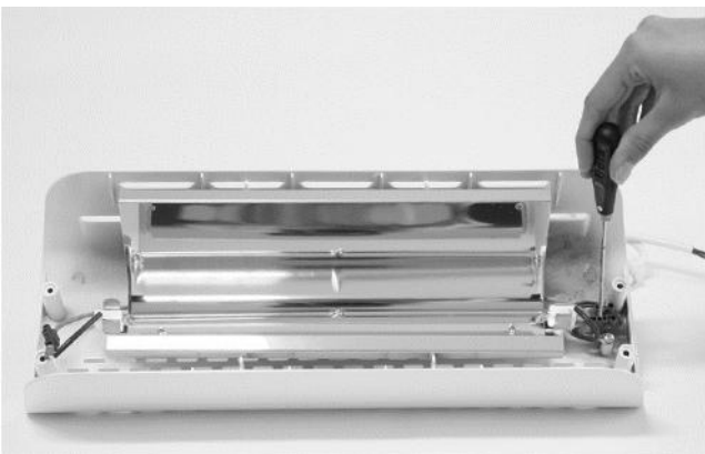
3. REMOVE THE FRONT COMPONENT OF THE DEVICE. UNSCREW THE SCREWS OF THE CLAMPS TO WHICH THE TWO BULB CORDS ARE CONNECTED.
