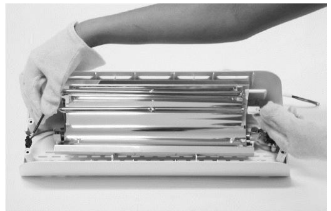
4. REMOVE THE BULB FROM THE SPRING CLIPS.
