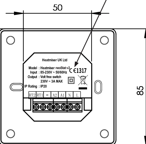
Wiring Detail
