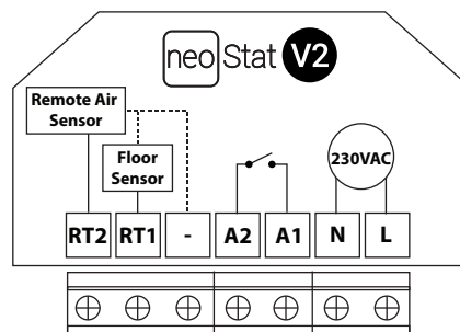
Wiring Detail
